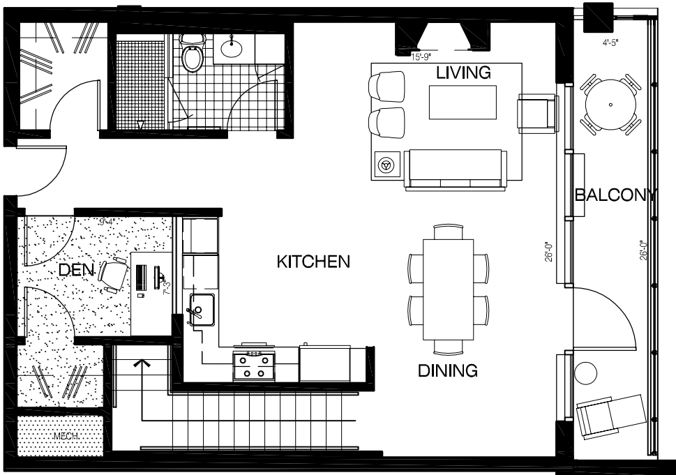
UPPER FLOOR
